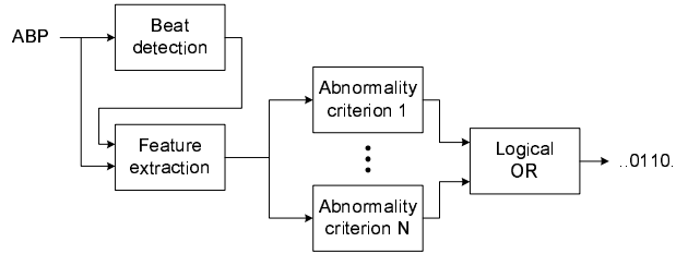
Figure 2. SAI block diagram. Input is an ABP waveform. Output is a binary string, assigning a value (no flag=0, flag=1) to each beat in the ABP waveform.
